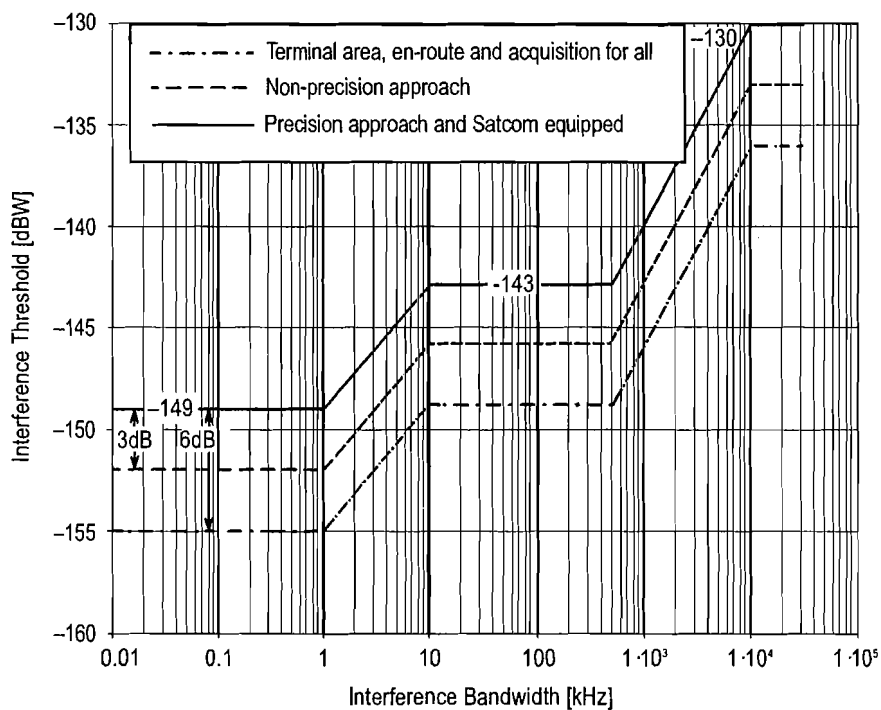
Figure B-18. Interference thresholds versus bandwidth for GLONASS
