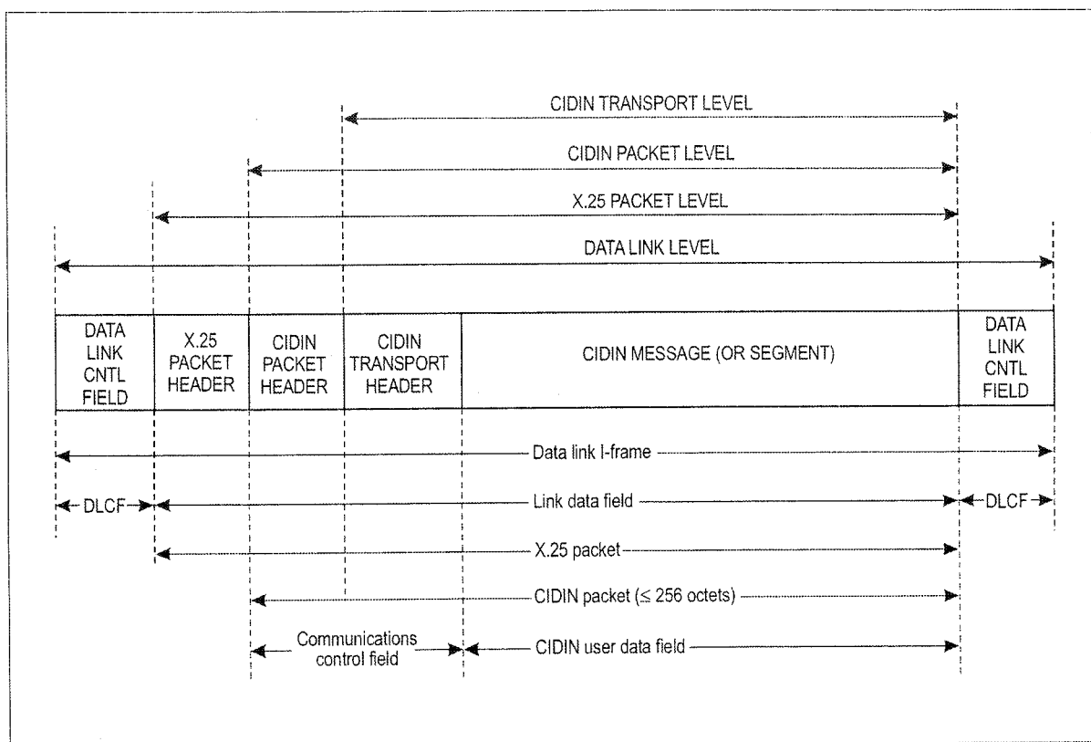
Figure 8-2. CIDIN terminology
