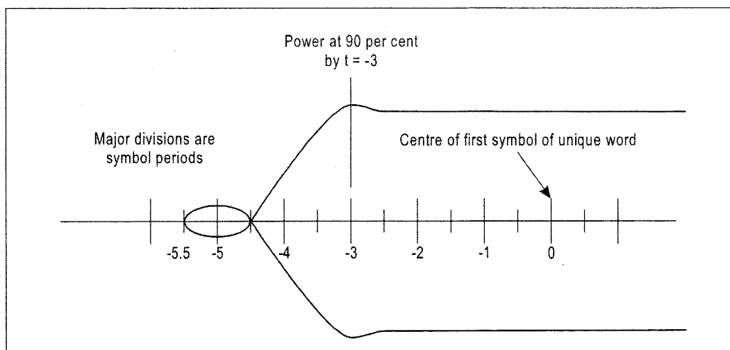
Figure 6-1. Transmitter power stabilization
