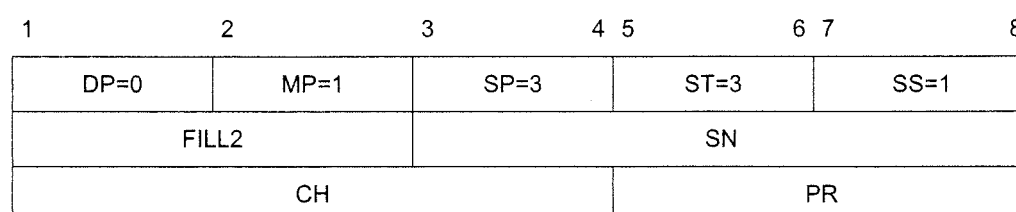
Figure 5-14. REJECT packet
