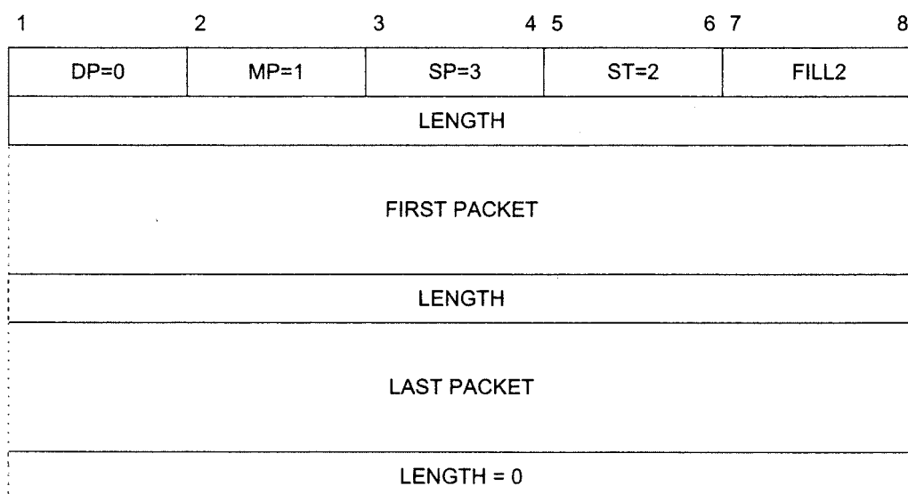
Figure 5-20. MULTIPLEX packet
