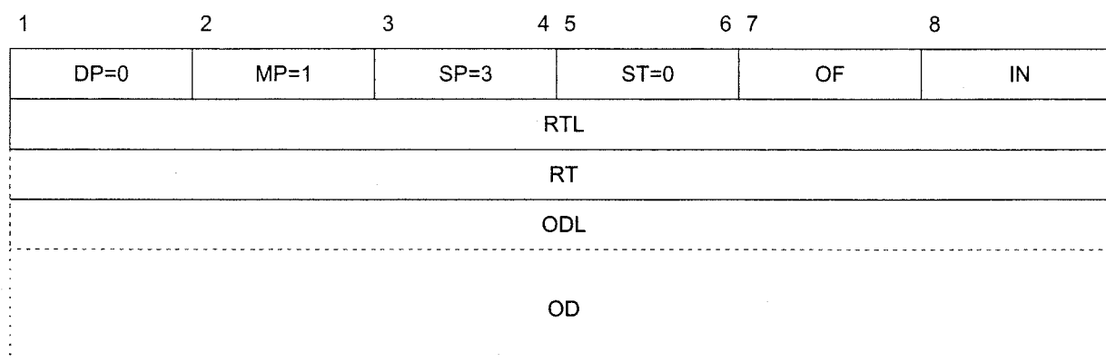
Figure 5-19. ROUTE packet
