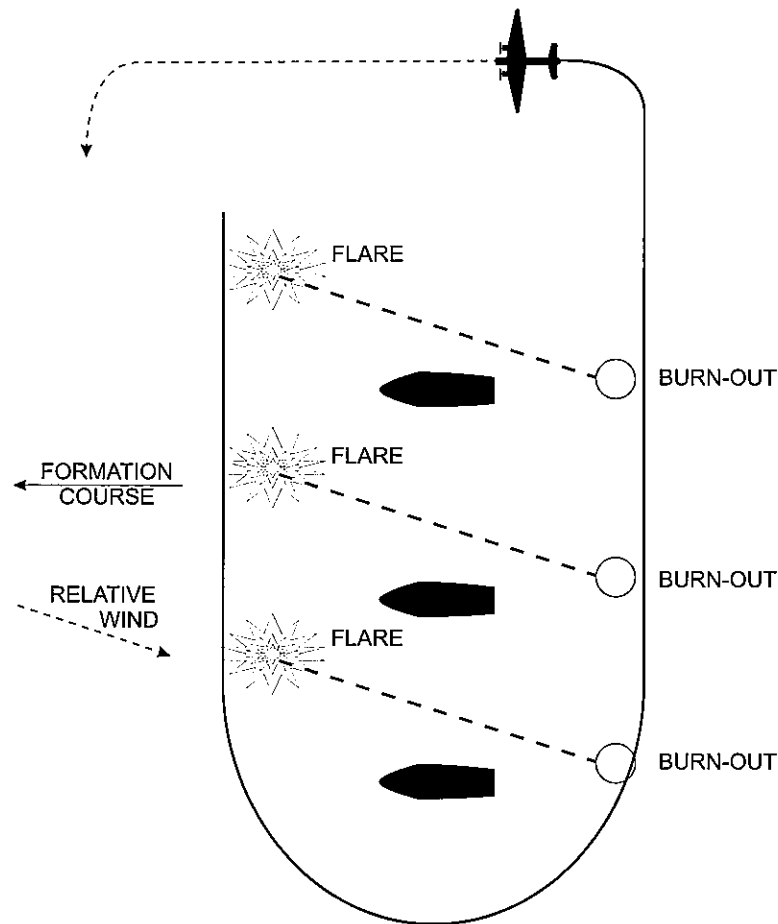
Figure 5-17 – Parachute flare search using several surface facilities
