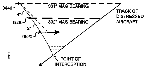
Figure J-5 - Offset or beam-on intercept: method 3
