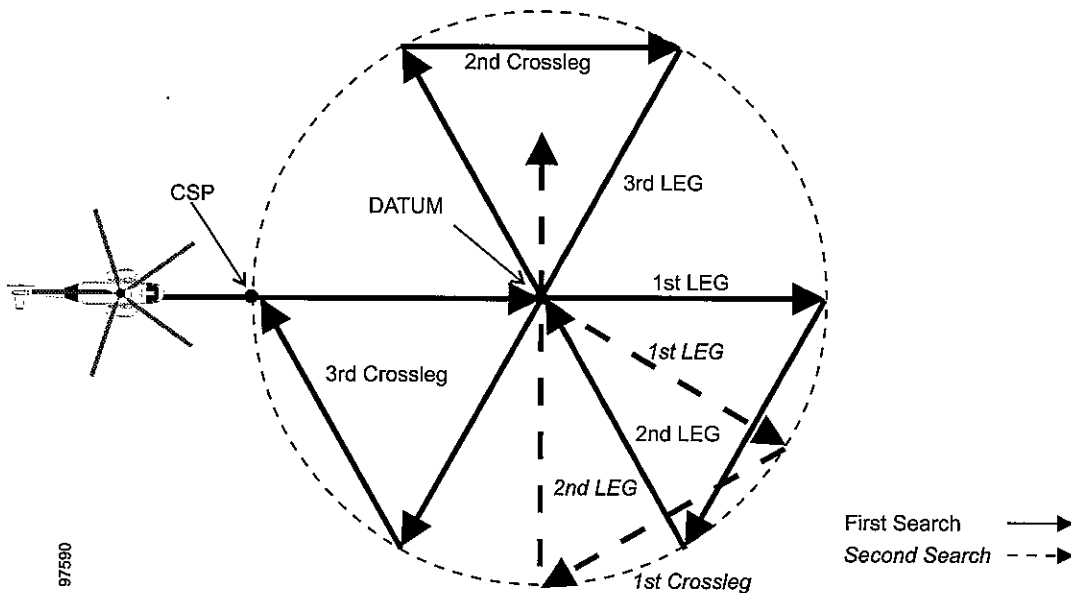
Figure 5-1 – Sector pattern: single-unit
