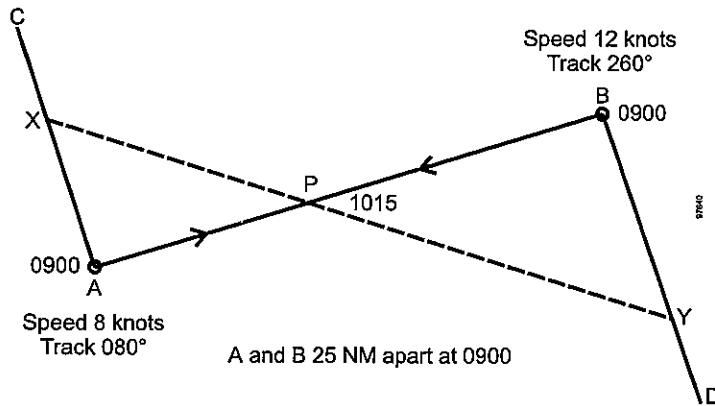
Figure J-1 - Head-on method
