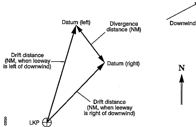
Figure K-1a – Drift velocity vectors with leeway divergence
