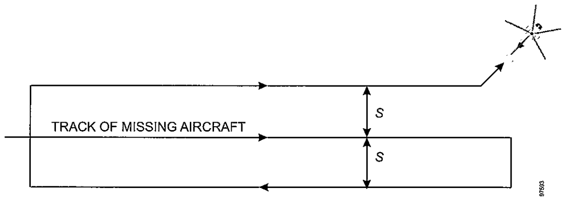
Figure 5-4 – Track line search, return (TSR)
